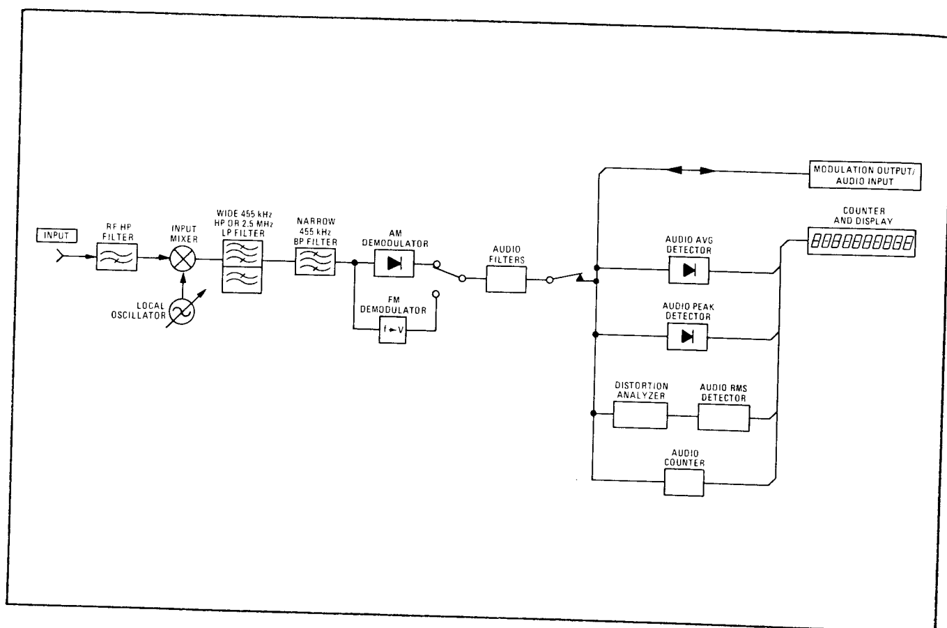
Audio Filters Block Diagram
