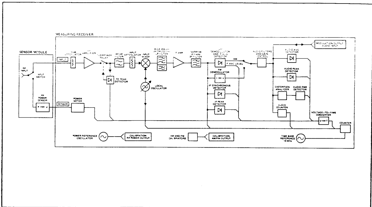
Figure 1-2. HP 8902A Measuring Receiver Simplified Block Diagram
