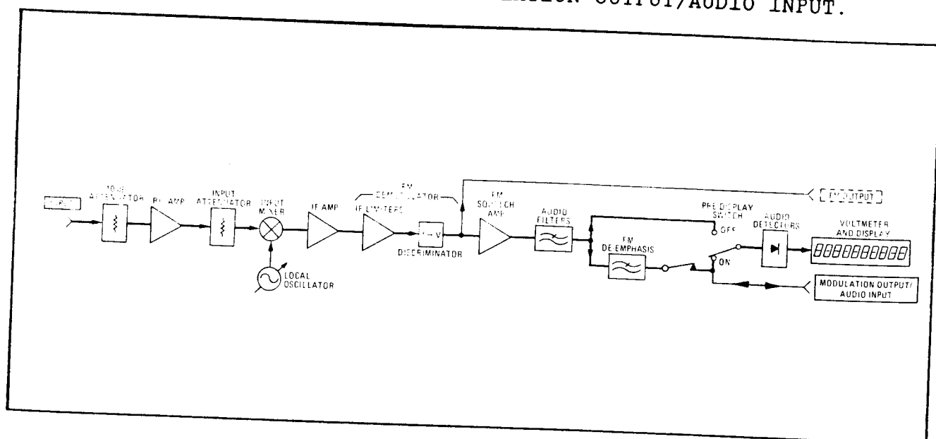
FM Measurement Block Diagram
