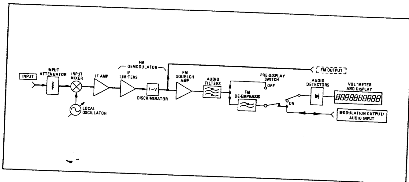
FM OUTPUT Block Diagram
