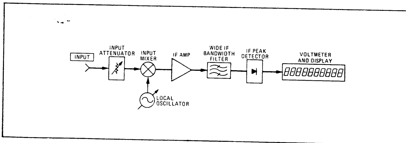
Peak Tuned RF Level Measurement Block Diagram
