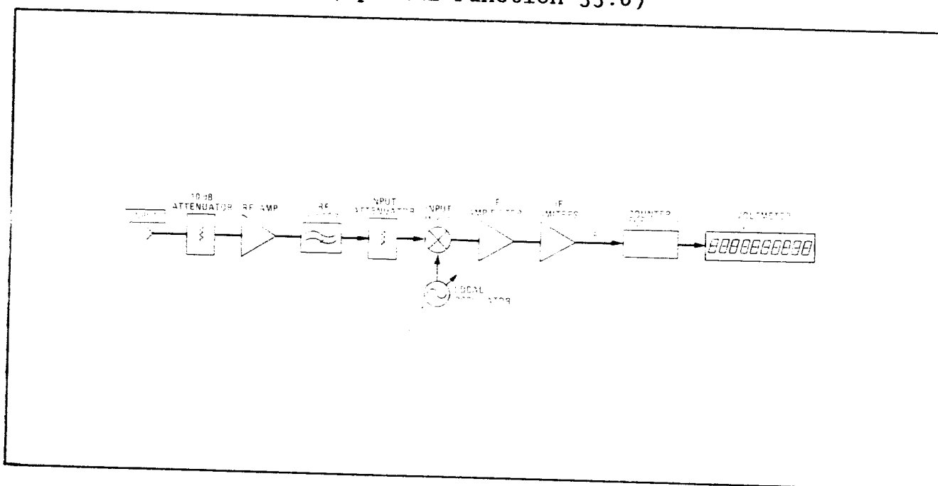
LO Frequency Measurement Block Diagram
