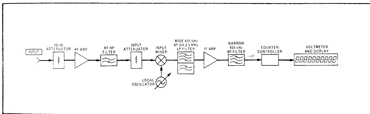
Block Diagram of RF and IF Filters
